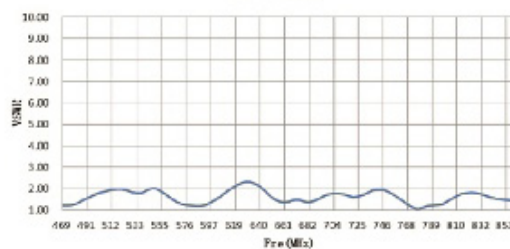
UHF VSWR
