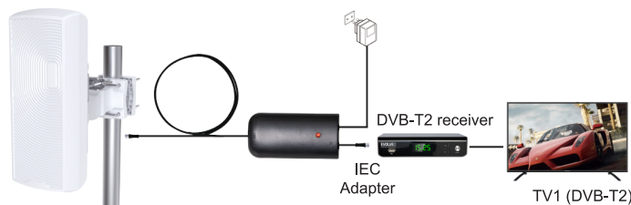
Installation 2: Connected through set-top box (Fig.7)
